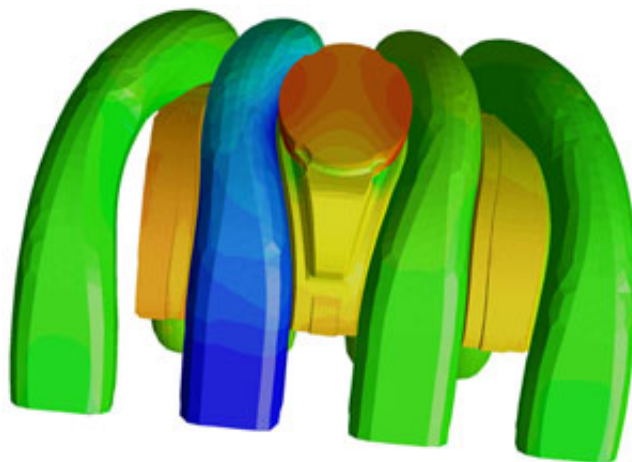
Pressure contours on a multi-head automotive plenum model. Graphic courtesy of Fluent.
